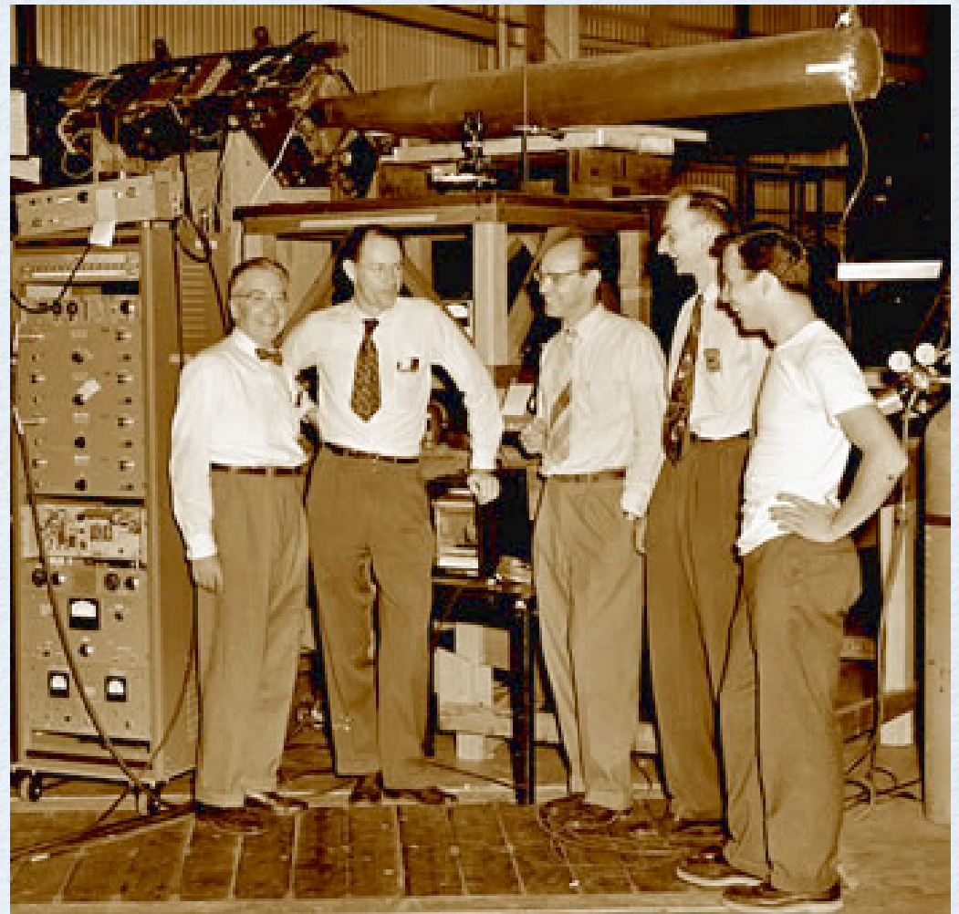
From left, Emilio Segrè, Clyde Wiegand, Edward Lofgren, Owen Chamberlain, and Thomas Ypsilantis, members of the team that discovered the antiproton
